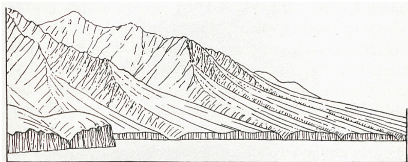
Fig. 8—Center Hill, on the northwest coast of Montserrat, showing the deeply incised inner valleys between sharply serrated ridges, the moderately dissected lower slopes, and the low cliffs of the shore. The higher cliffs in the left foreground are part of Silver Hill, Fig. 6.
