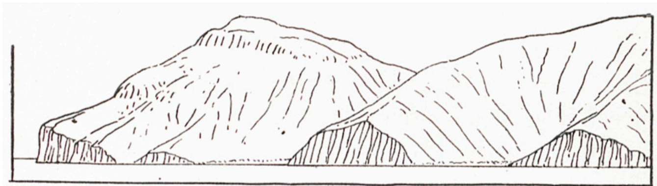
Fig. 38—Cliffed headlands west of Kingstown harbor, southern end of St. Vincent.
